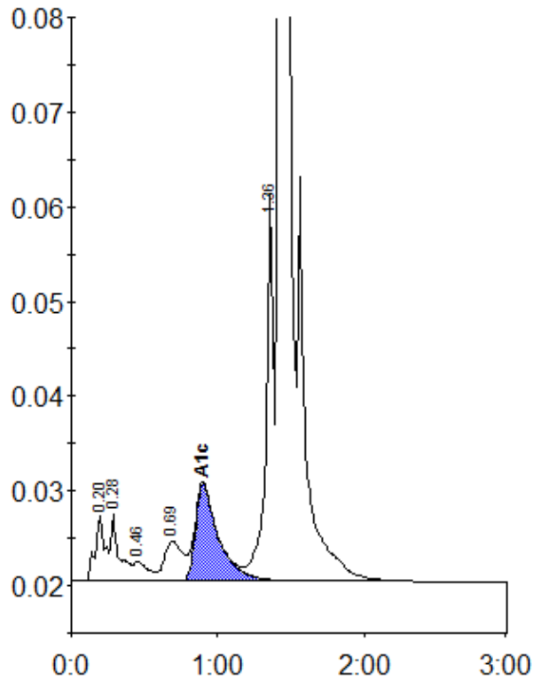
Peak table - ID: 10583411
